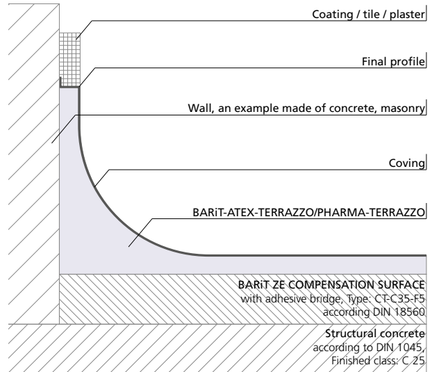
Coving composite construction
