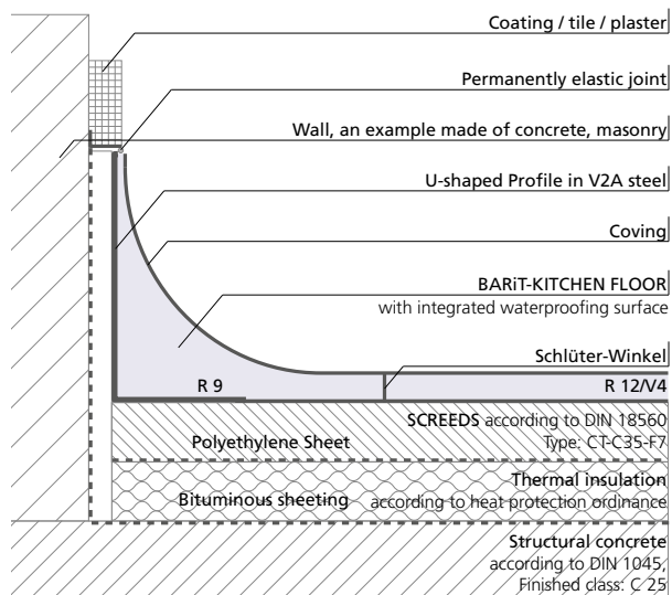
Coving construction on isolation
