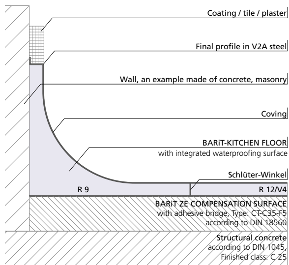
Coving composite construction
